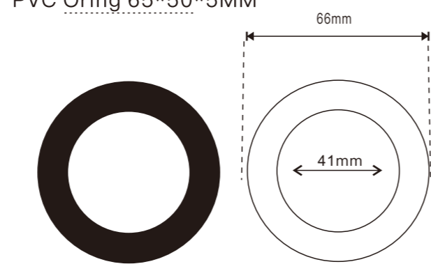
DW-23 PVC Oring 66*41*1MM
