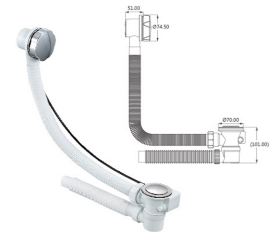
DT-1004 Bathtub Drain
