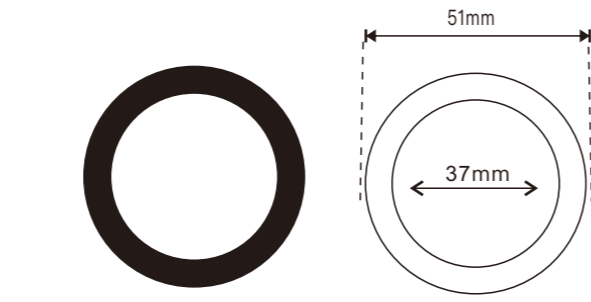
DW-19 PVC Oring 51*37*1MM
