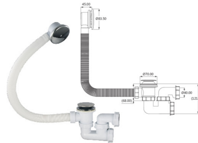
DT-1003 Bathtub Drain
