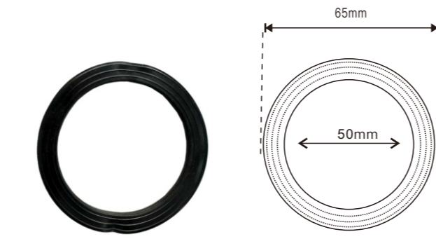
DW-21 PVC Oring 65*50*5MM
